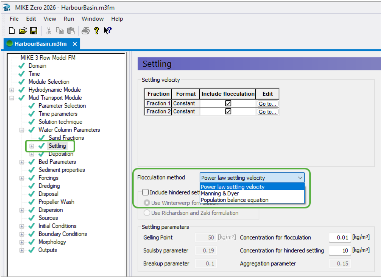
Figure 2 – Flocculation methods in Mud Transport module
